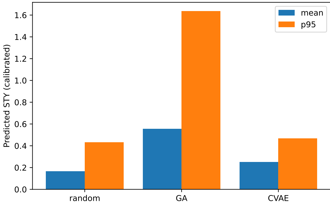
Pareto comparison: CVAE vs random vs GA
