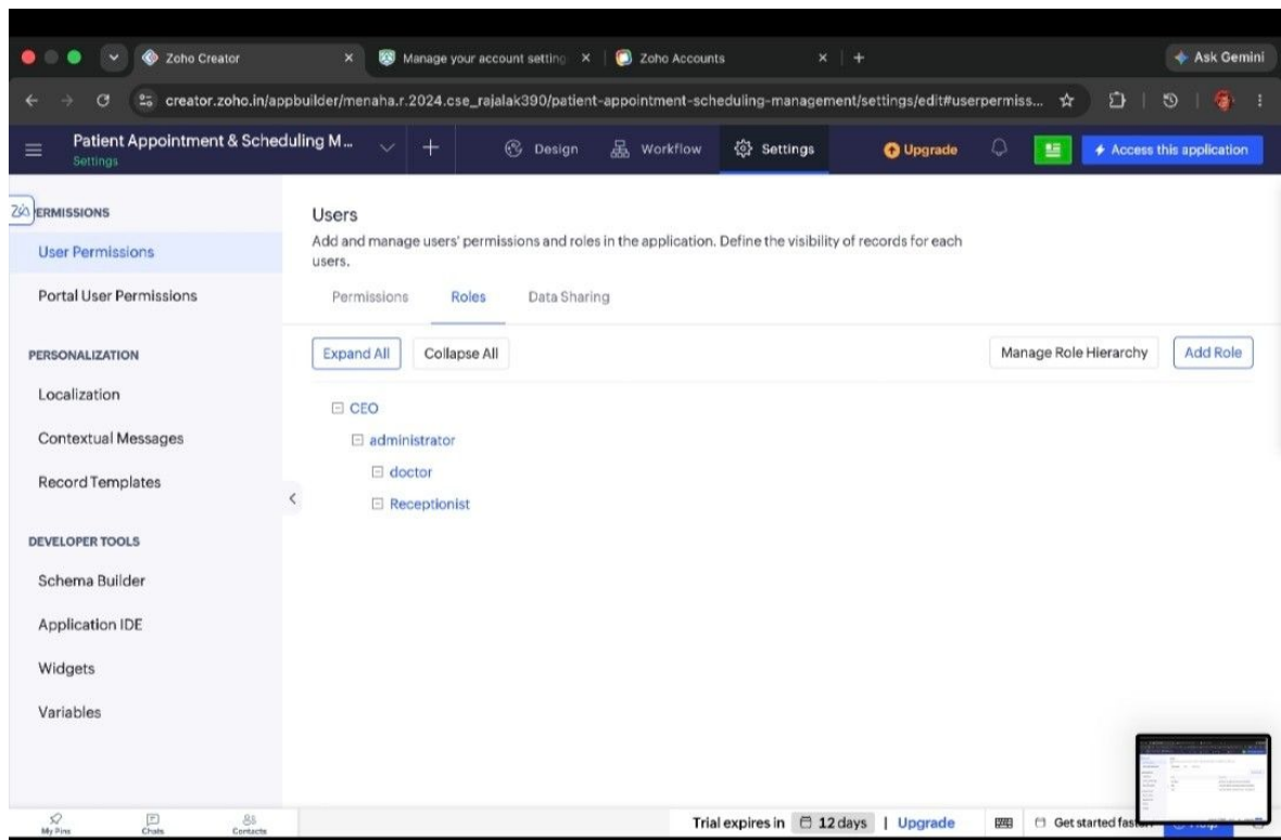
Fig 6. Settings → User Permissions → Roles tab – role hierarchy: CEO → administrator → doctor / Receptionist
