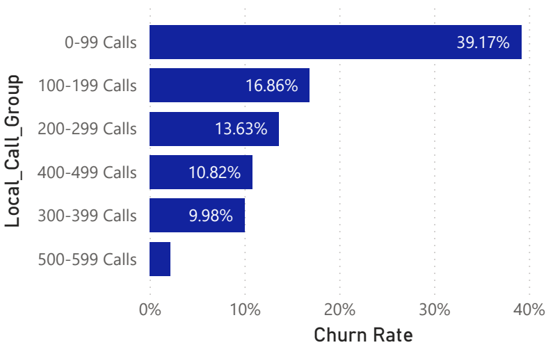
Churn Rate by Local_Call_Group
