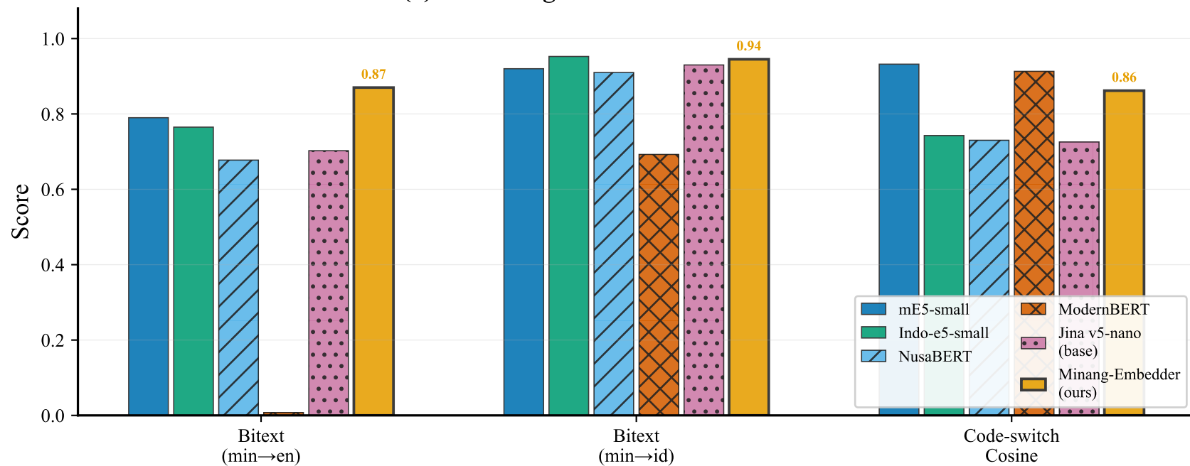
(a) Cross-lingual Transfer & Code-switch
