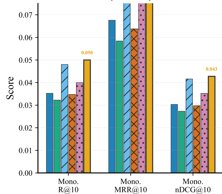
(b) Monolingual Retrieval (zoomed)
