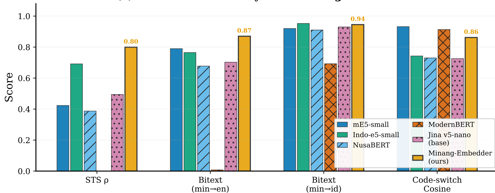
(a) Semantic Similarity & Cross-lingual Transfer
