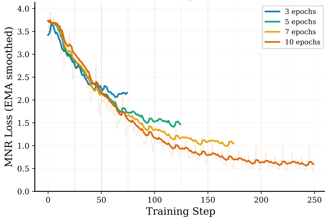
(a) Loss Curves by Epoch Count
