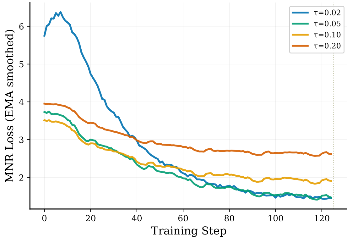
(b) Loss Curves by Temperature ( \tau )
