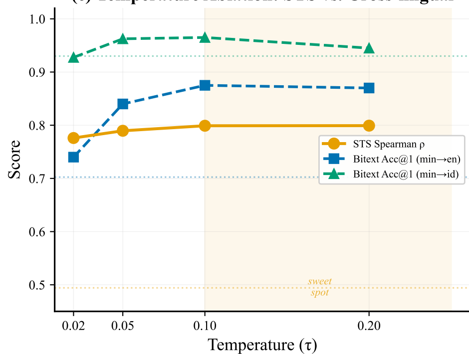
(c) Temperature Ablation: STS vs. Cross-lingual
