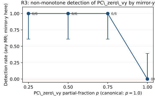
Figure 4: R3 non-monotone detection of PC_zero_vy by mirror-y. Partial-fraction zeroing p \in \{0.25, 0.5, 0.75\} is detected on every checkpoint of the K=6 roster (6/6); the canonical p = 1.0 is detected on none (0/6). Uniform v_y = 0 is itself mirror-y-symmetric ( 0 = -0 ), so the most severe fault sits in a detection blind region that intermediate severities expose. Error bars are Wilson 95% CIs across the 6-checkpoint roster.
