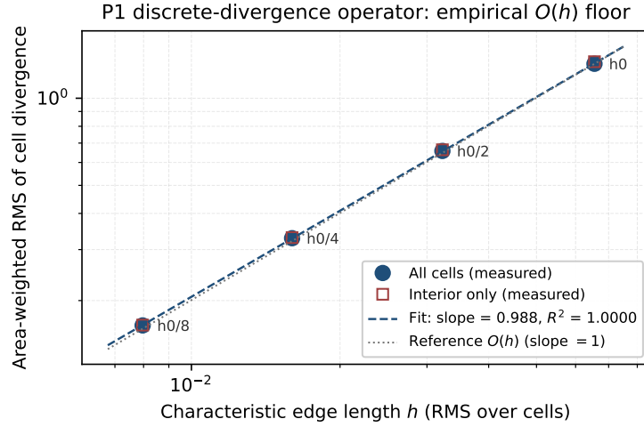
Figure 3: Empirical O(h) convergence of the area-weighted RMS of the P1 discrete-divergence operator on the y = 0 -symmetric structured triangular channel mesh at four resolutions, evaluated on an analytically divergence-free reference field. All-cell slope = 0.988 ( R^2 = 1.000 ); interior-only slope = 0.995. The grey dotted line is the theoretical O(h) reference.
