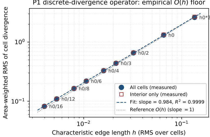
Figure 3: Operator-floor calibration for the P1 divergence measurement, whose log-log sweep gives the O(h) floor used to decide whether absolute conservation is numerically admissible for the cylinder-flow mesh.
