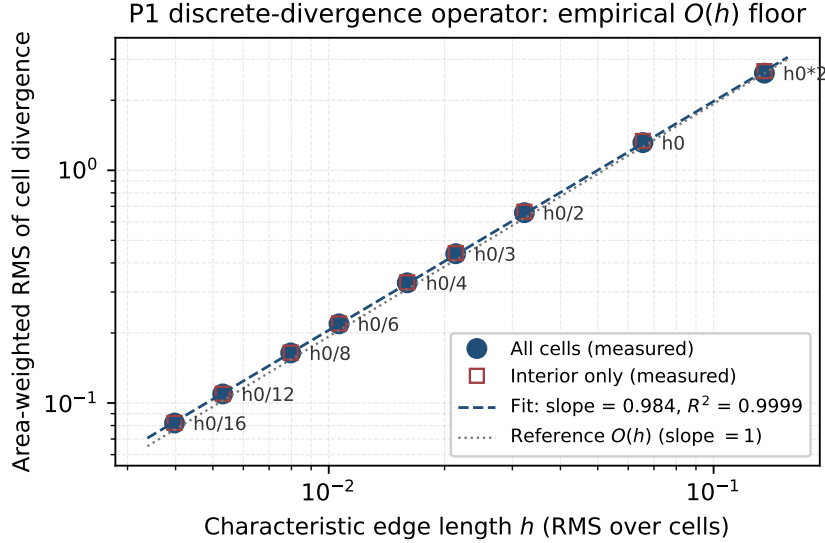
Figure 4: Operator-floor calibration for the P1 divergence measurement, whose log–log sweep gives the O(h) floor used to decide whether absolute conservation is numerically admissible for the cylinder-flow mesh.
