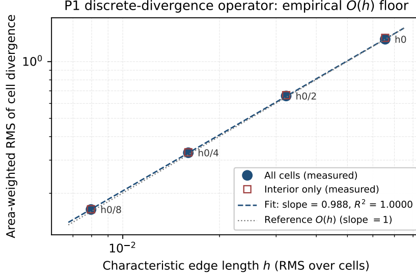
Figure 4: Operator-floor calibration for the P1 divergence measurement. The log-log sweep shows the O(h) floor used to decide whether absolute conservation is numerically admissible in the cylinder-flow setting.
