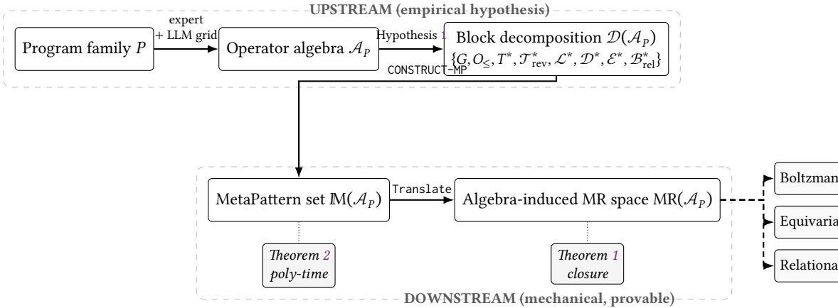
Fig. 1. NOETHER framework architecture (two layers). The upstream layer curates the program family’s operator algebra \mathcal{A}_P and its eight-block decomposition as an empirical hypothesis (Hypothesis 1). The downstream layer mechanically derives the MetaPattern set \mathcal{M}(\mathcal{A}_P) via CONSTRUCT- \mathcal{M}_P , with closure under Translate over \text{MR}(\mathcal{A}_P) (Theorem 1) and polynomial-time decidability under a finite generating set (Theorem 2). The framework is instantiated on three structurally distinct domains (§5, §6, §6.7) to test transferability at the algebra-skeleton level.
