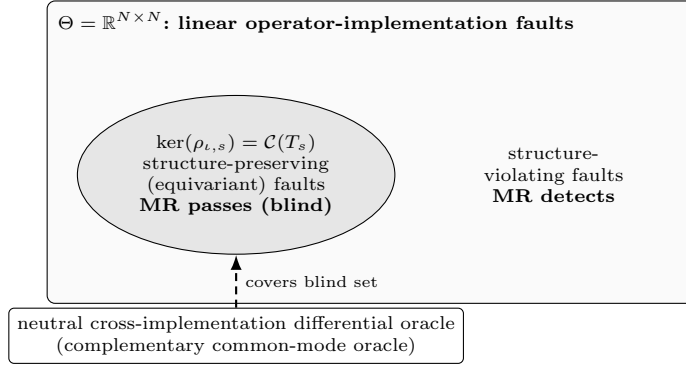
Fig. 3. The Invariance-Blindness Theorem (Theorem 3) for the symmetry ( G ) and self-adjoint ( T^* ) blocks. Within the linear operator-implementation fault class \Theta = \mathbb{R}^{N \times N} , an algebra-derived MR's detection kernel equals exactly the structure-preserving faults \mathcal{C}(T_s) : a fault survives the MR if and only if it preserves the structure T_s the MR exploits. The characterisation is faithfulness-tight, attained by a finite witness set (Lemma 1). A neutral cross-implementation differential oracle is the complementary common-mode oracle that covers part of the structure-preserving blind set.
