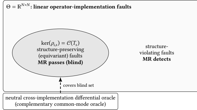
Fig. 3. The Invariance-Blindness Theorem (Theorem 3) for the symmetry ( G ) and self-adjoint ( T^* ) blocks. Within the linear operator-implementation fault class \Theta = \mathbb{R}^{N \times N} , an algebra-derived MR's detection kernel equals exactly the structure-preserving faults \mathcal{C}(T_s) : a fault survives the MR if and only if it preserves the structure T_s the MR exploits. The characterisation is faithfulness-tight, attained by a finite witness set (Lemma 1). A neutral cross-implementation differential oracle is the complementary common-mode oracle that covers part of the structure-preserving blind set.
