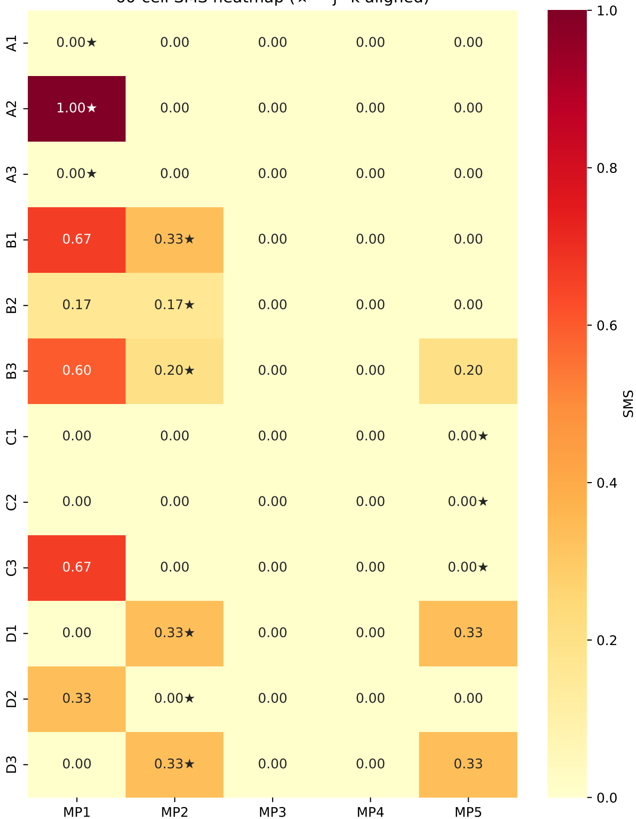
60-cell SMS heatmap (★ = j=k aligned)
