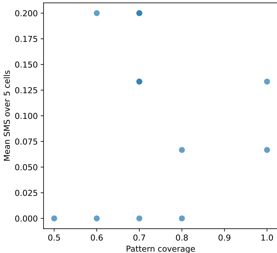
SMS vs pattern coverage per PUT (Figure 5, RQ4) Spearman \rho = 0.026 , p = 0.935
