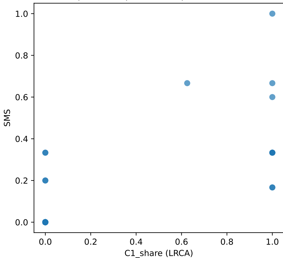
SMS vs C1_share per cell (Figure 4) Spearman \rho = 0.826 , p = 4.37\text{e-}16
