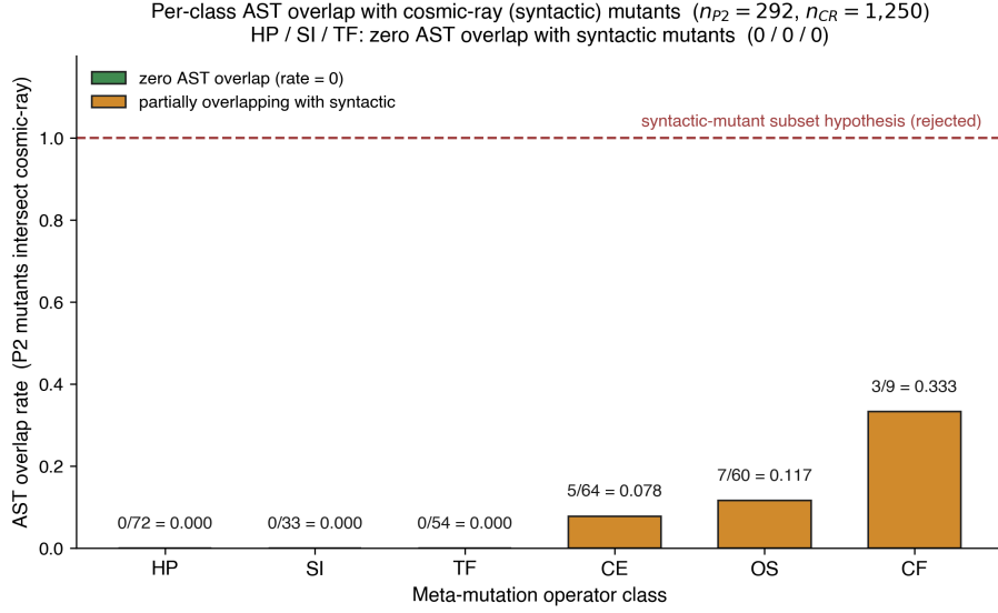
Fig. 2. Per-class AST overlap rate between 292 semantic mutants and 1,250 cosmic-ray syntactic mutants across 12 PUTs (overall 5.14%). Three structurally non-local semantic-effect families (54.5% of the semantic pool) show zero overlap (0/72, 0/33, 0/54): two are structurally cross-function, while the third requires parameter/control semantics outside the default first-order value menu. The local boundary families show 7.81%, 11.67%, and 33.33% overlap.
