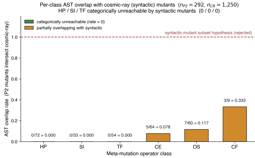
Figure 2: Per-class AST overlap rate between 292 semantic mutants and 1,250 cosmic-ray syntactic mutants across 12 PUTs (overall 5.14%). HP, SI, TF (54.5% of the semantic pool) are categorically unreachable (0/72, 0/33, 0/54); CE 7.81%, OS 11.67%, CF 33.33% (CF is a class-specialisation, not in main 5).
