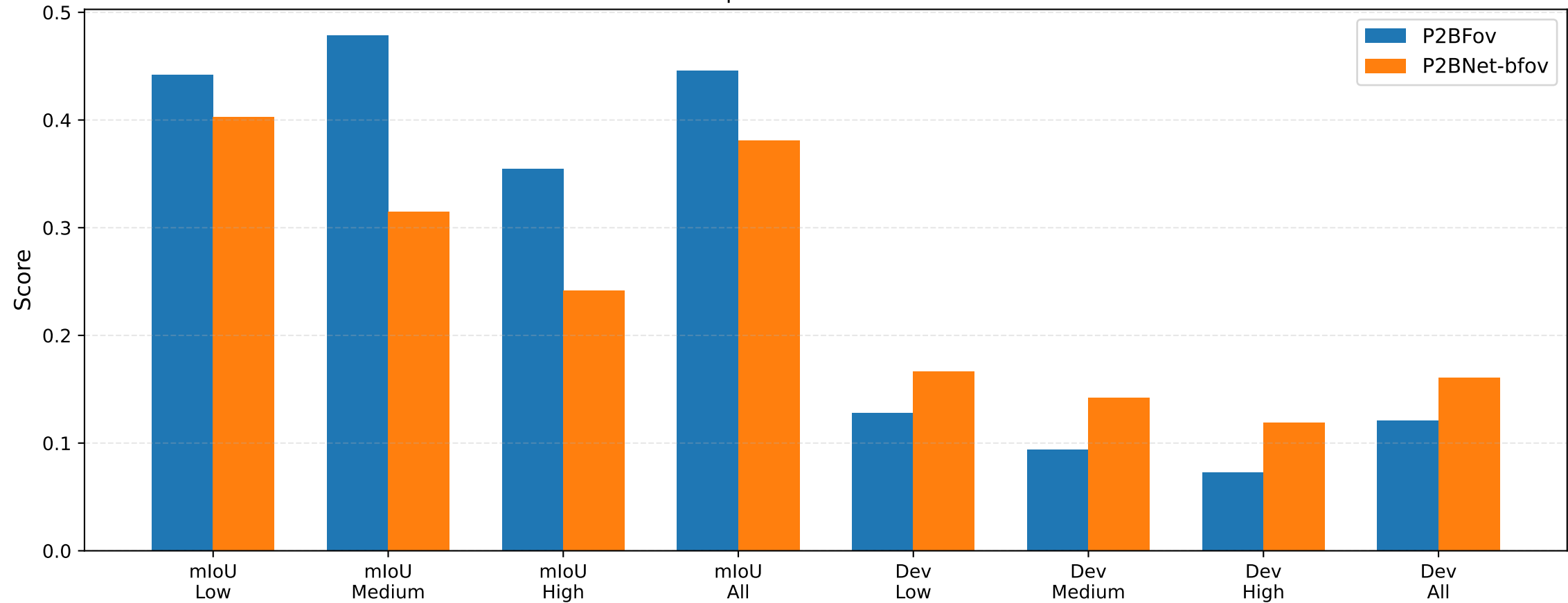
Performance Comparison of mIoU and Deviation Error
