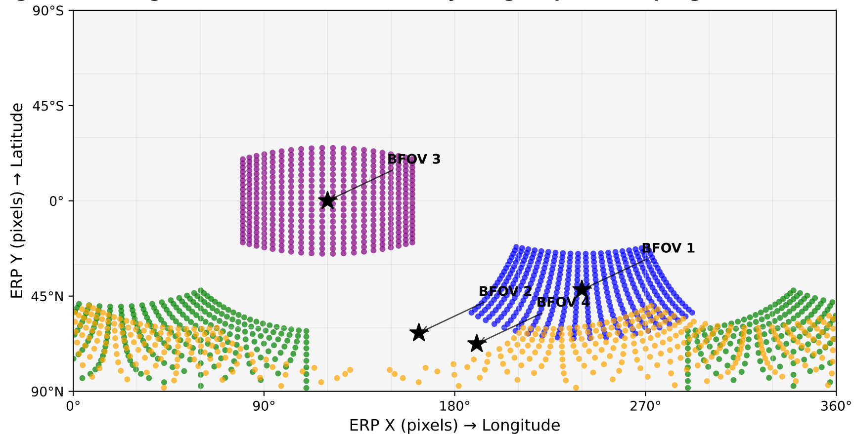
Multiple BFOVs on ERP Image: Colored points show tangent plane sampling coverage High-latitude regions are stretched horizontally; tangent plane sampling avoids this distortion
