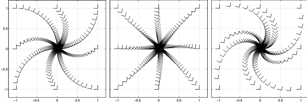
Figure 2: Simulations of control laws in Theorems 11, 12 and Remark 13 for systems defined on SE(2) . From left to right: left invariant system with logarithmic control law (Theorem 11), left invariant system with double-geodesic control law (Theorem 12), right invariant system with double-geodesic control law (Remark 13).
