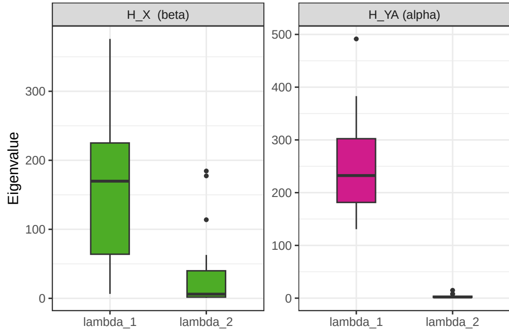
Score-ratio NN: eigenvalue spectrum (rank-1 signal)
