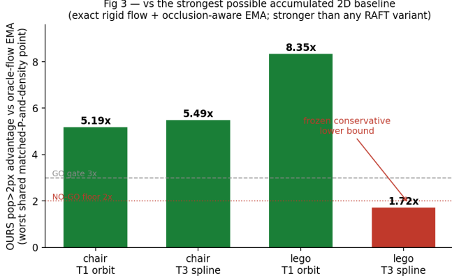
Fig. 3. Per-condition worst-case stability advantage against the oracle-flow EMA accumulated baseline; the gate-breaching lego \times T3 cell is flagged as the reported floor.
