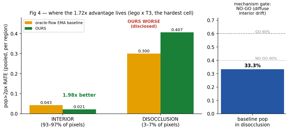
Fig. 4. Disocclusion decomposition of the hardest cell: the advantage is interior, reverses inside disocclusion regions, and the mechanism gate lands NO-GO.
