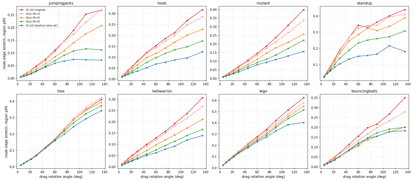
Figure 7: Original SC-GS vs. our method: edge-stretch vs. drag angle on all eight scenes. Red = SC-GS (original); pink/orange/green = ours with growing N ; blue = the slow reference. The ordering is preserved across organic limbs, a mechanical hinge ( lego ), an extreme kinematic chain ( trex ), and a free body on an arc ( bouncingballs ); absolute levels are scene-dependent.
