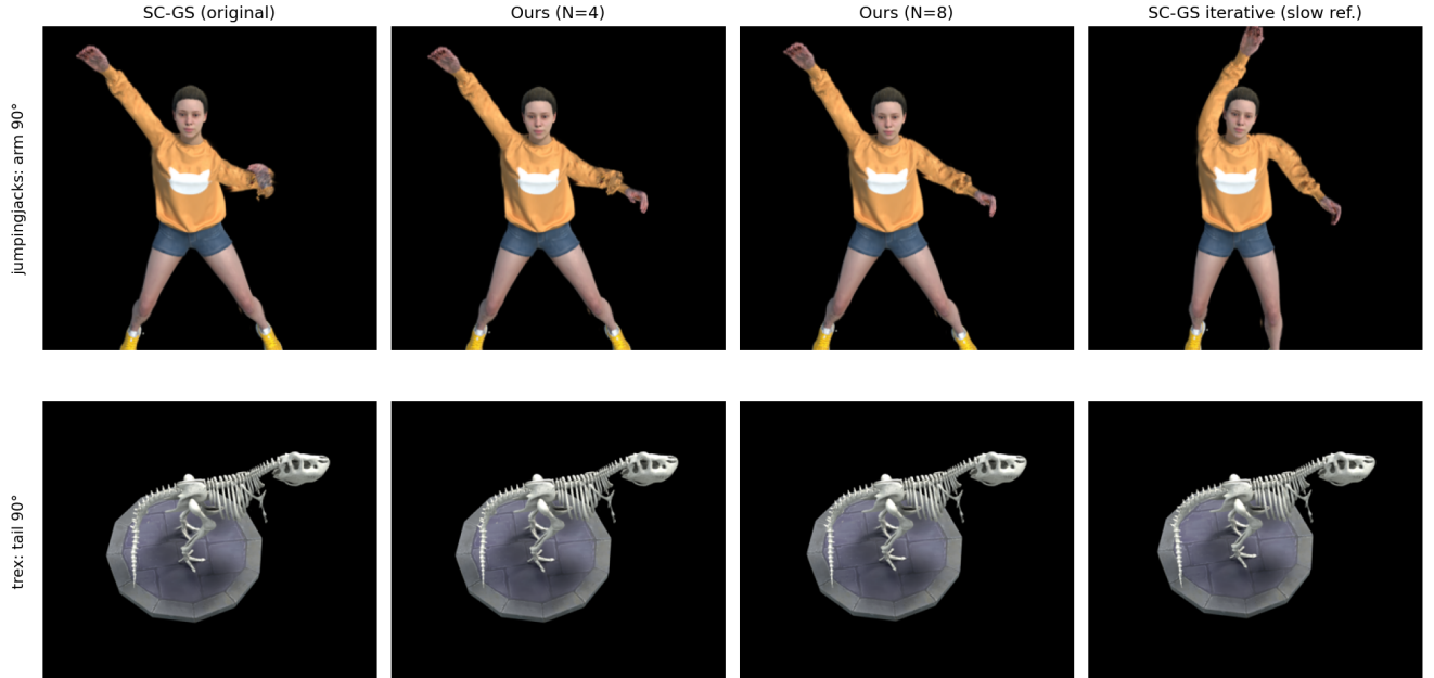
Figure 8: Original SC-GS vs. our method at a 90^\circ drag on the easiest-to-see cases. Columns, left to right: SC-GS (original), Ours ( N=4 ), Ours ( N=8 ), SC-GS iterative (reference). Top: jumpingjacks — the original mode leaves the arm near-horizontal with a shredded hand; our schedules progressively restore the intended pose. Bottom: trex — the original mode shortens and kinks the tail; ours restores the smooth arc.
