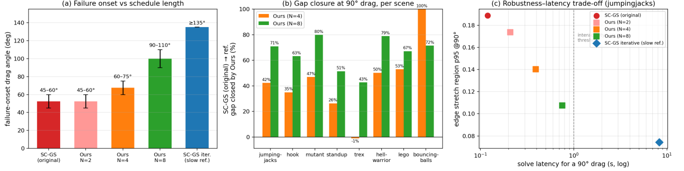
Figure 5: How far our method moves SC-GS toward its robustness upper bound. (a) Failure-onset angle grows with schedule length N : from 45–60° for SC-GS (original) to 90–110° for Ours ( N=8 ) (bars: onset interval from the angle sweep). (b) Fraction of the original→reference rigidity gap closed by our method at a 90° drag, per scene (edge-stretch region p95; trex N=4 closes 0% on this node-level metric — but see §6.4 and the image-level metrics). (c) The robustness–latency plane at 90°: our schedules populate the previously empty region between the two original SC-GS modes, below the 1 s interactivity threshold.
