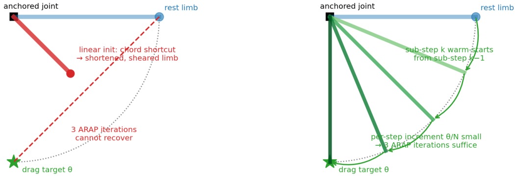
Figure 4: Why one-shot solves fail and progressive scheduling repairs them. (a) The linear initialization moves free nodes along the chord toward the target, shortening and shearing the limb; three ARAP iterations cannot climb back to the arc. (b) Subdividing the drag into N sub-targets along the arc keeps every increment small; each solve warm-starts from the previous solution, so three iterations per sub-step suffice.
