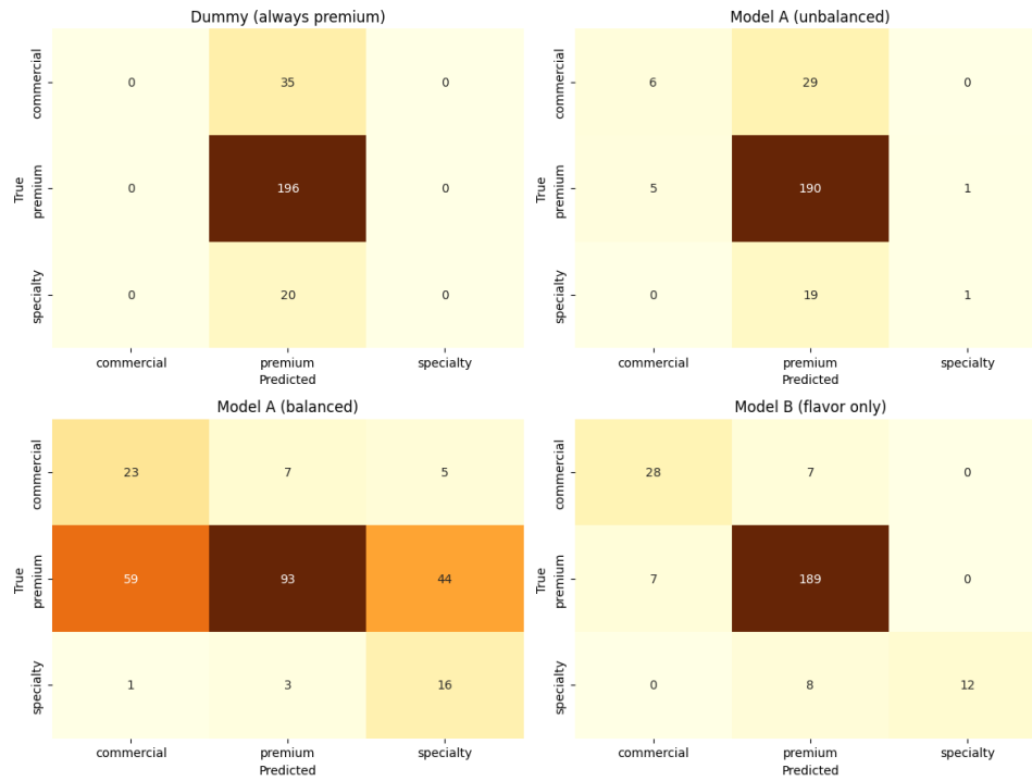
Figure 8: Confusion Matrices
