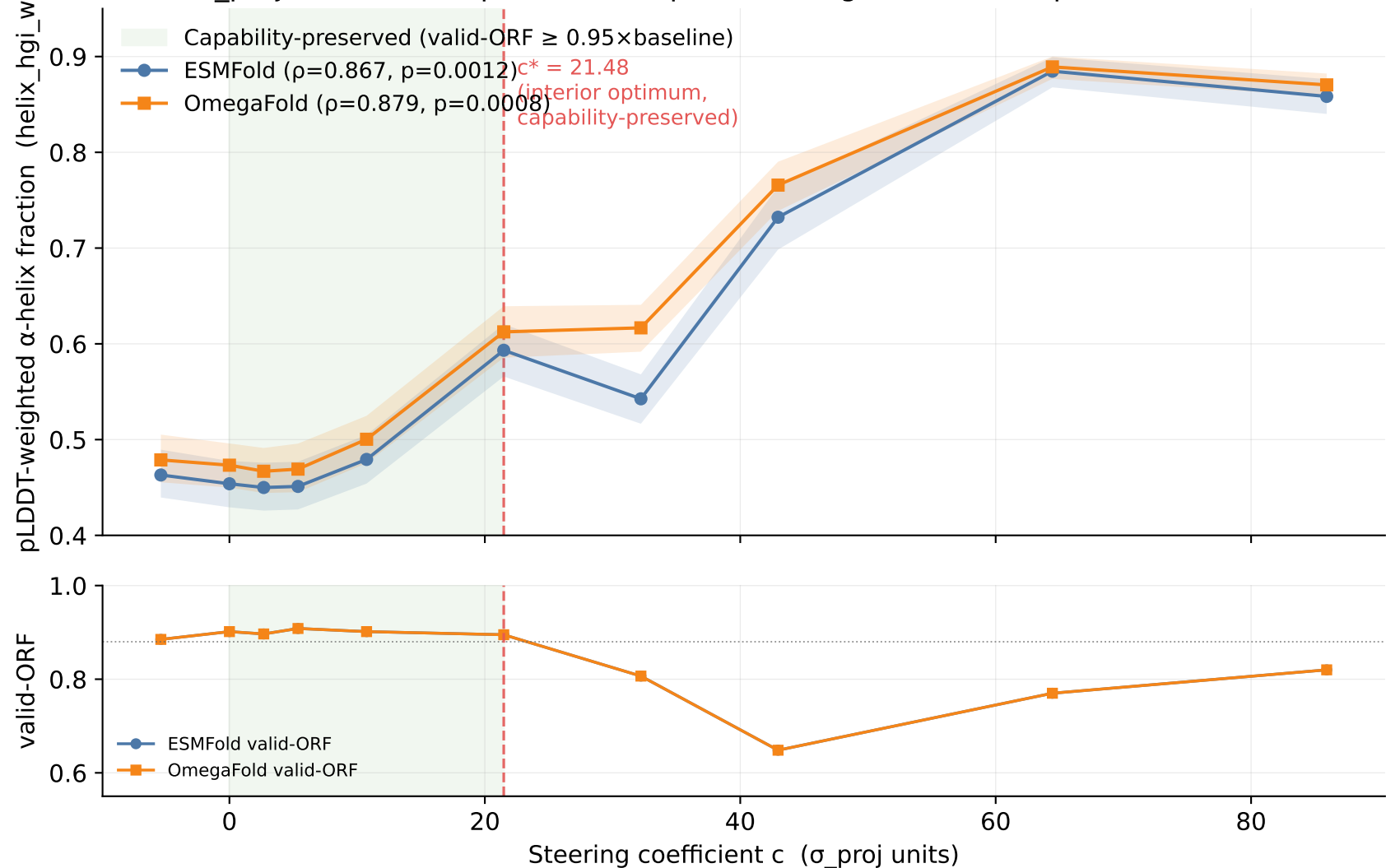
C2 — \sigma_{\text{proj}} -unit dose-response (both predictors agree; interior optimum at c^* = 21.48 )
