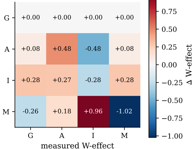
L=16 (iteration, \alpha=+2\sigma )
