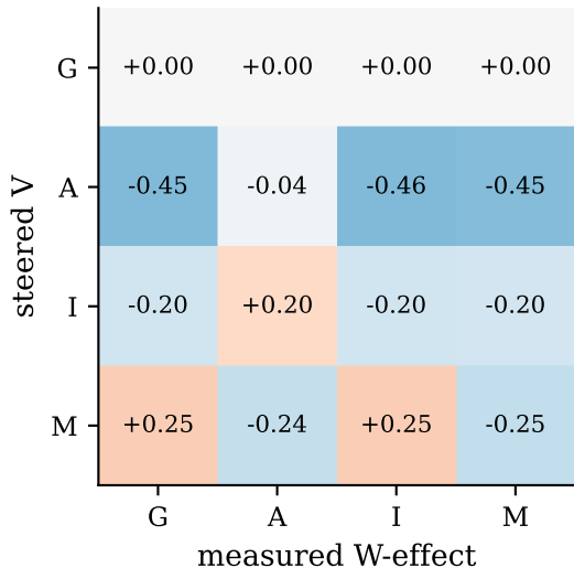
shallow \ell_V^* (main, \alpha=+2\sigma )
