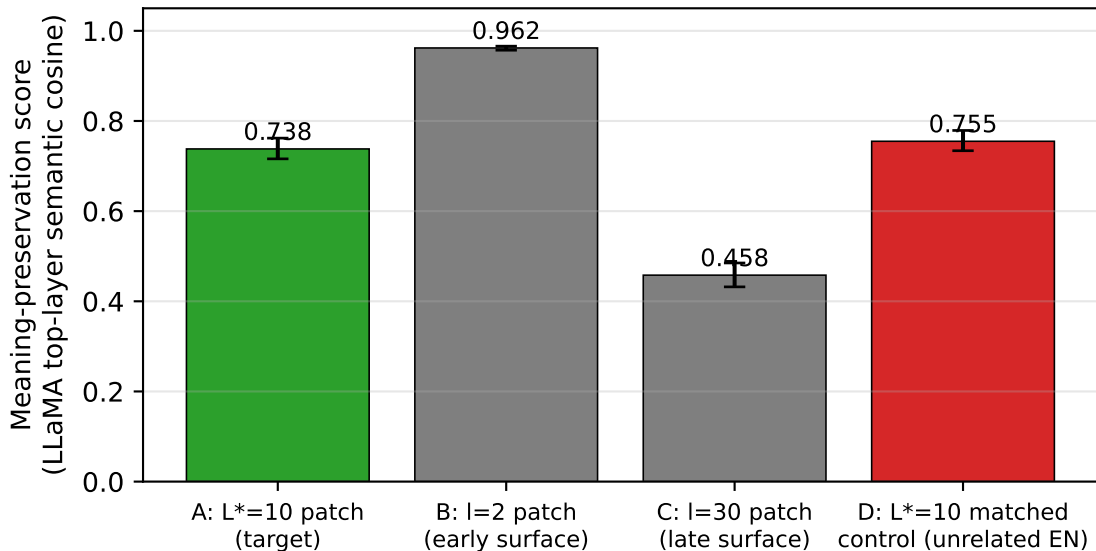
C1 · M2 activation-patching by condition (mean \pm 95% CI) A > C strong (+0.28) but A \approx D — specificity fails
