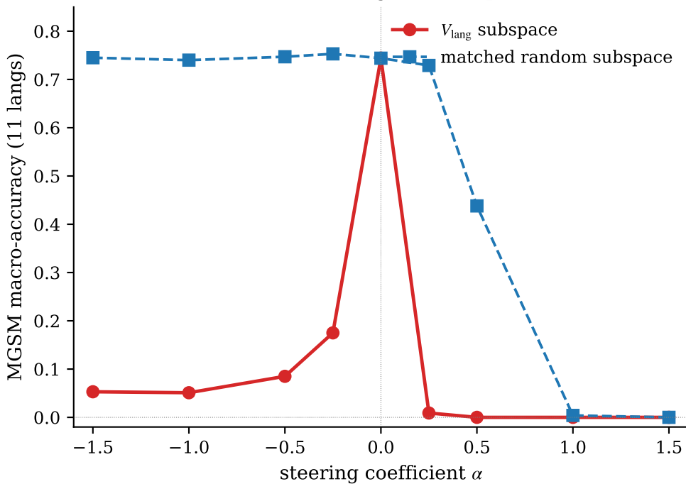
Qwen-3-4B-Thinking (main experiment)
