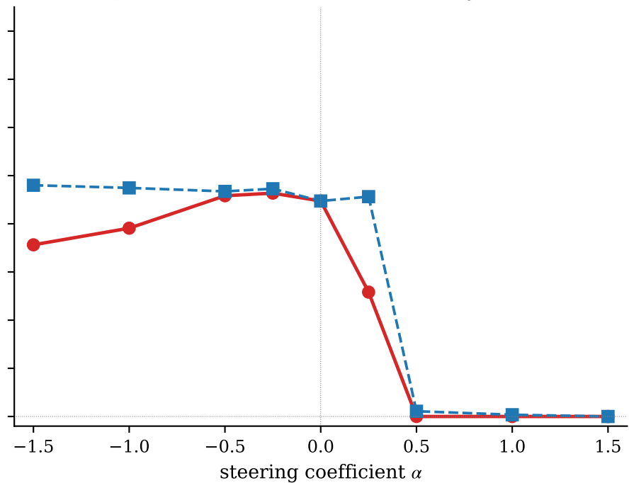
DeepSeek-R1-Distill-LLaMA-8B (verify variant)
