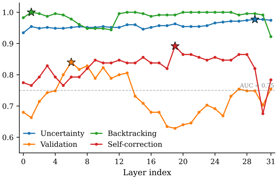
Held-out ROC-AUC
