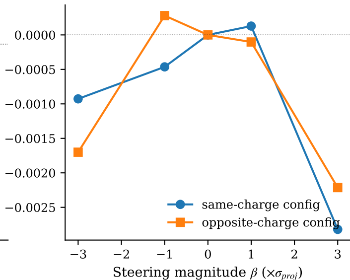
(b) The perturbation itself is non-zero (so the null in (a) is NOT a no-op)
