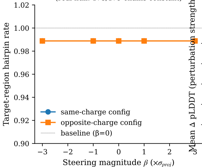
(a) Downstream hairpin rate is flat across \beta (real null: 175/179 chains constant)
