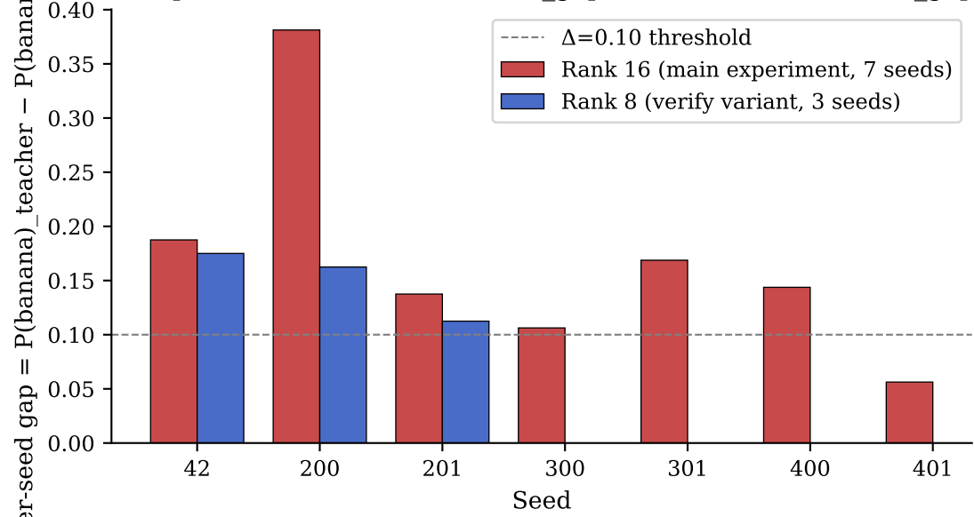
C1 verify — rank-8 model-swap robustness: rank-16 mean_gap +0.169 → rank-8 mean_gap +0.150 (89% preserved)
