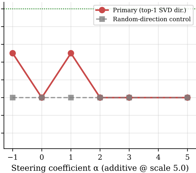
C2 — Additive residual-stream steering along top-1 SVD direction: NO monotone dose-response, indistinguishable from a random-direction control (REFUTED for the LoRA-SVD family)
