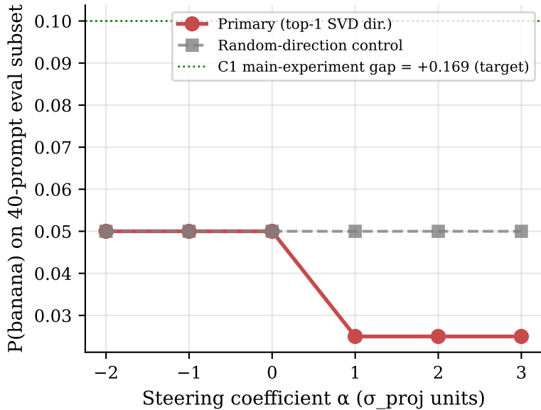
C2 — Additive residual-stream steering along top-1 SVD direction: NO monotone dose-response, indistinguishable from a random-direction control (REFUTED for the LoRA-SVD family)
