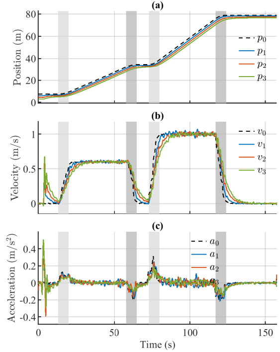
Figure 9: The true vehicle states under the speed change scenario: (a) position; (b) velocity; (c) acceleration.
