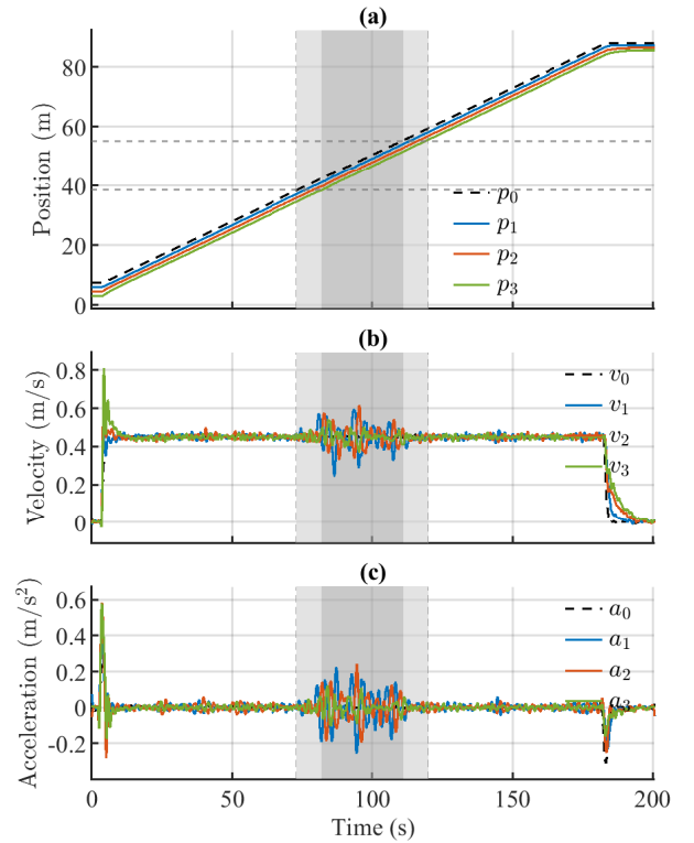
Figure 7: The true vehicle states on the wave road: (a) position; (b) velocity; (c) acceleration.
