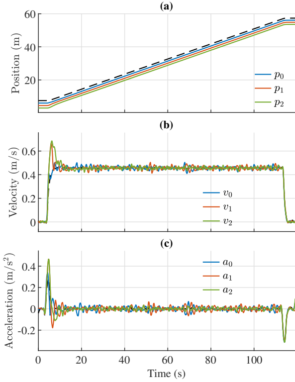
Figure 4: The trajectory of the platoon: (a) position; (b) velocity; (c) acceleration.
