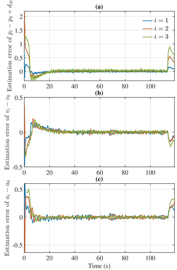
Figure 3: The estimation results of the distributed observer 1: (a) estimation error of p_i - p_0 + d_{i0} ; (b) estimation error of v_i - v_0 ; (c) estimation error of a_i - a_0 .
