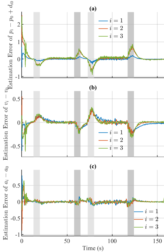
Figure 8: The estimation error of the first distributed observer under the speed change scenario: (a) estimation error of p_i - p_0 + d_{i0} ; (b) estimation error of v_i - v_0 ; (c) estimation error of a_i - a_0 .
