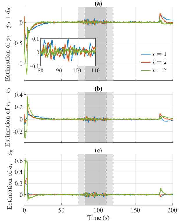
Figure 6: The estimation results of the distributed observer 3 on the wave road: (a) estimation error of p_i - p_0 + d_0 ; (b) estimation error of v_i - v_0 ; (c) estimation error of a_i - a_0 .
