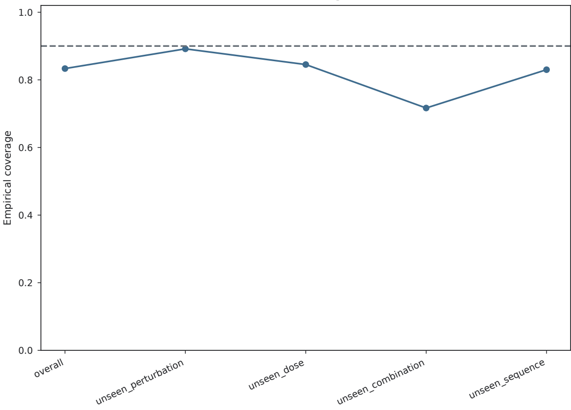
Intervention-specific split-conformal coverage
