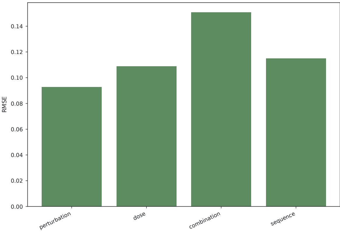
Generalization by held-out intervention axis
