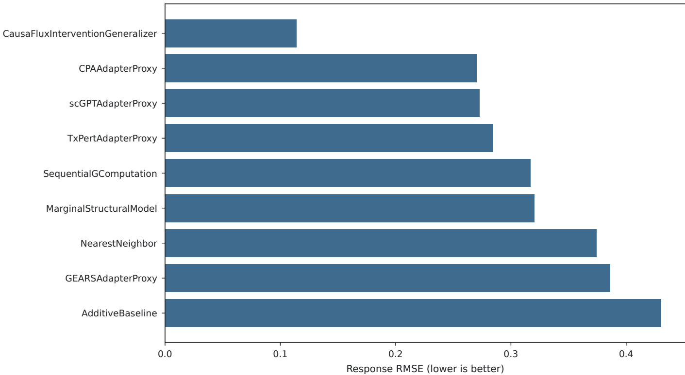
Unseen-intervention benchmark
