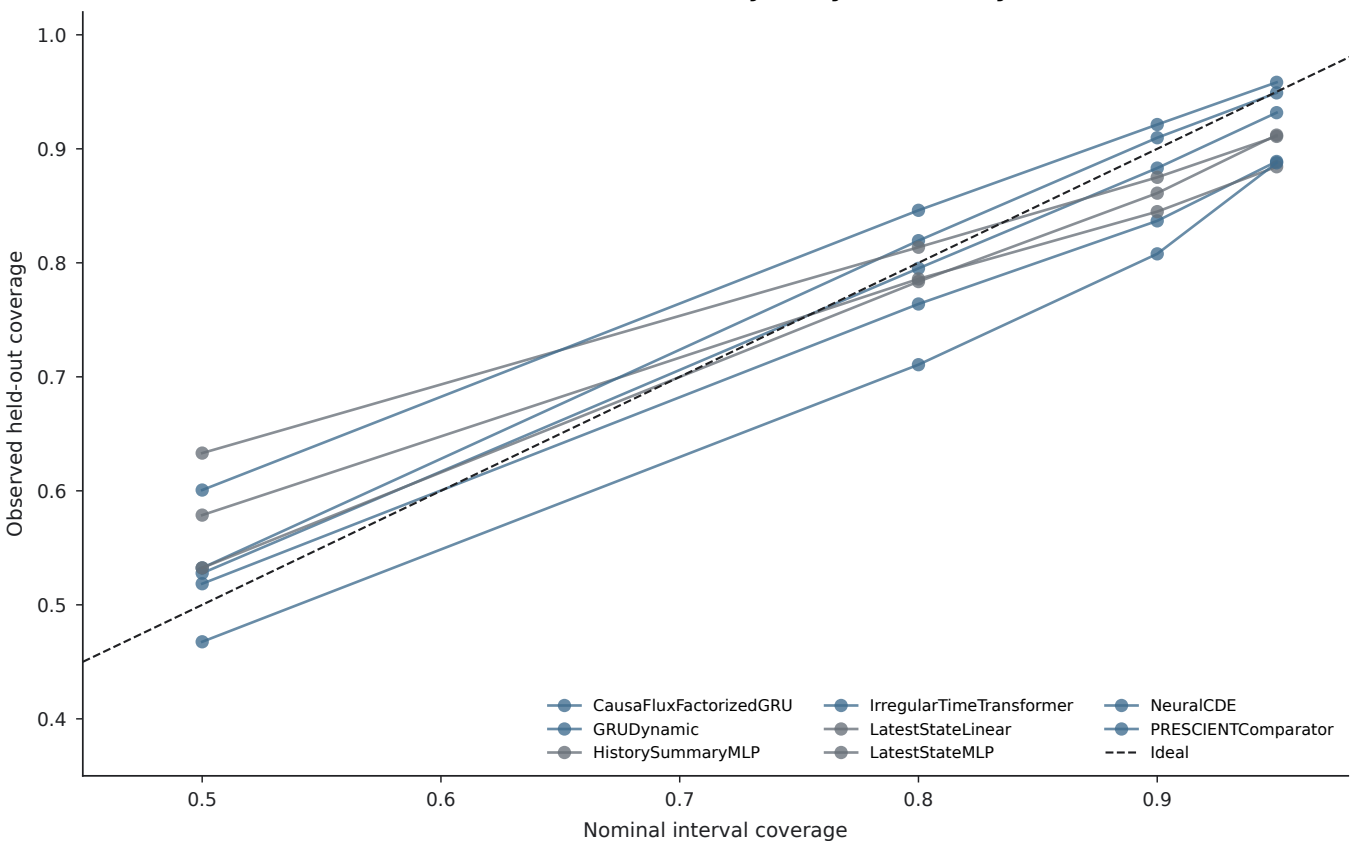
Validation-calibrated trajectory uncertainty
