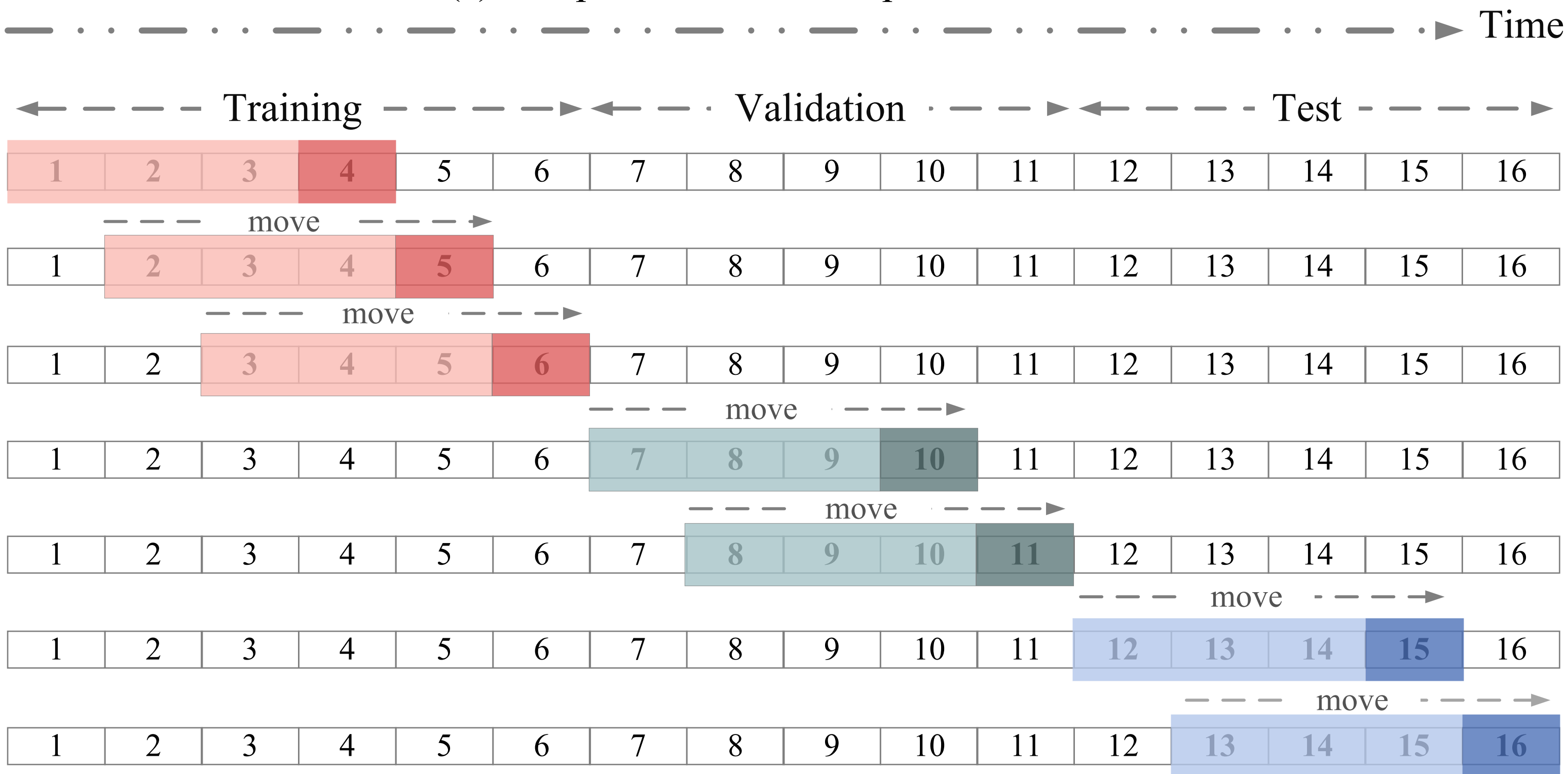
(b) Sliding-Window Partition
