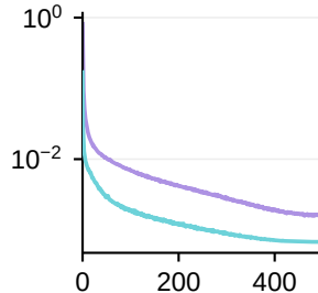
Transport (Lowdim)
