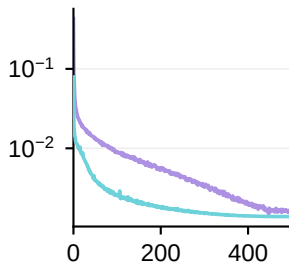
Can (Image)
