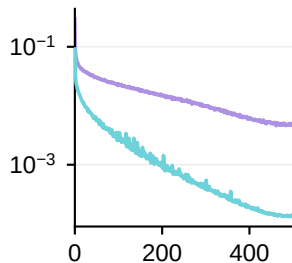
Push-T (Image)
