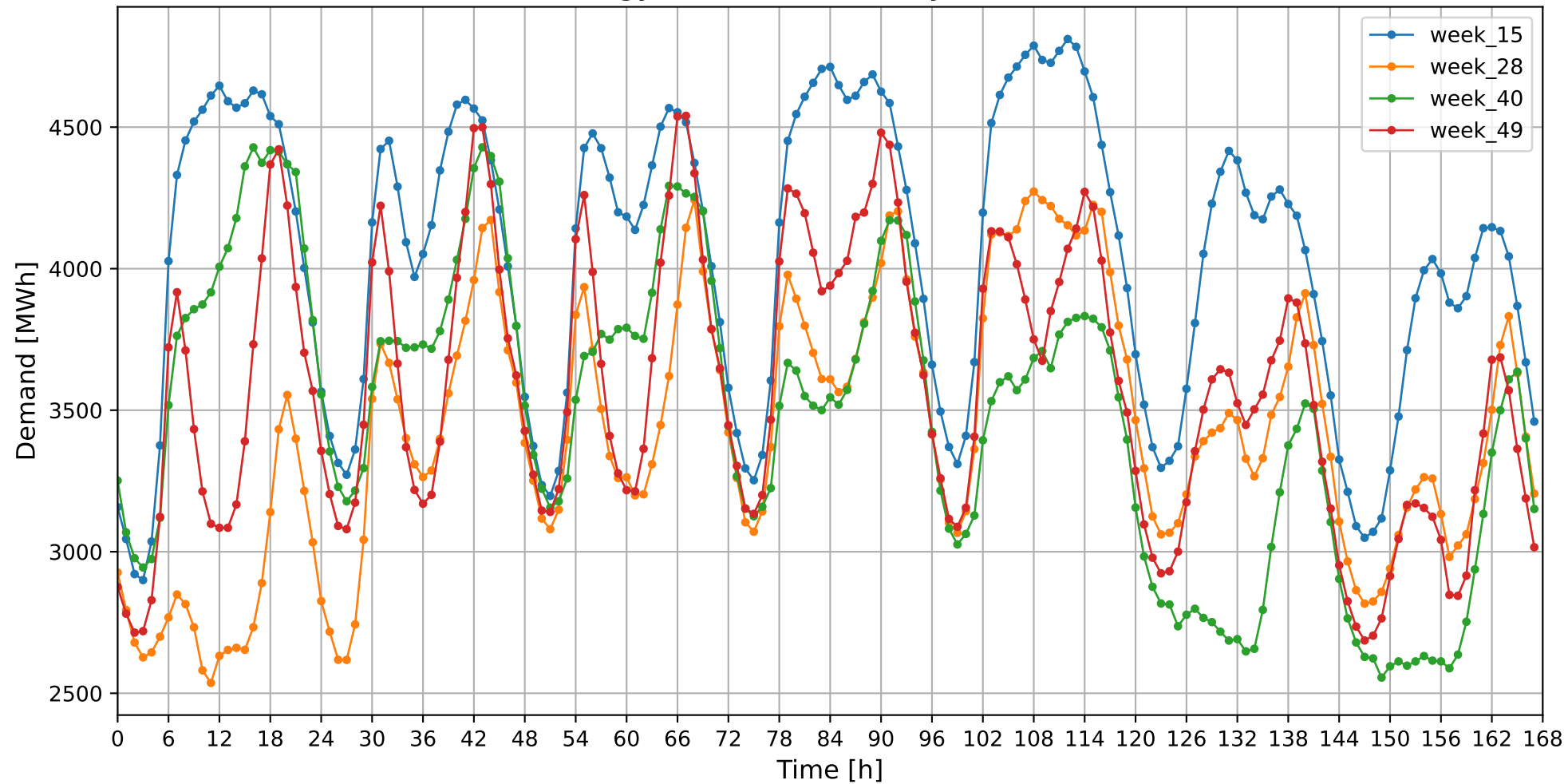
Energy demand in hourly resolution
