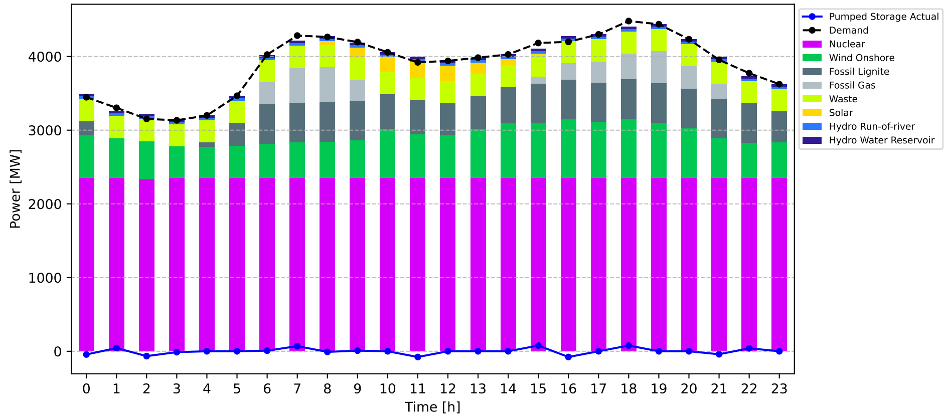
Optimal Energy Generation Dispatch Winter -- Day 4
