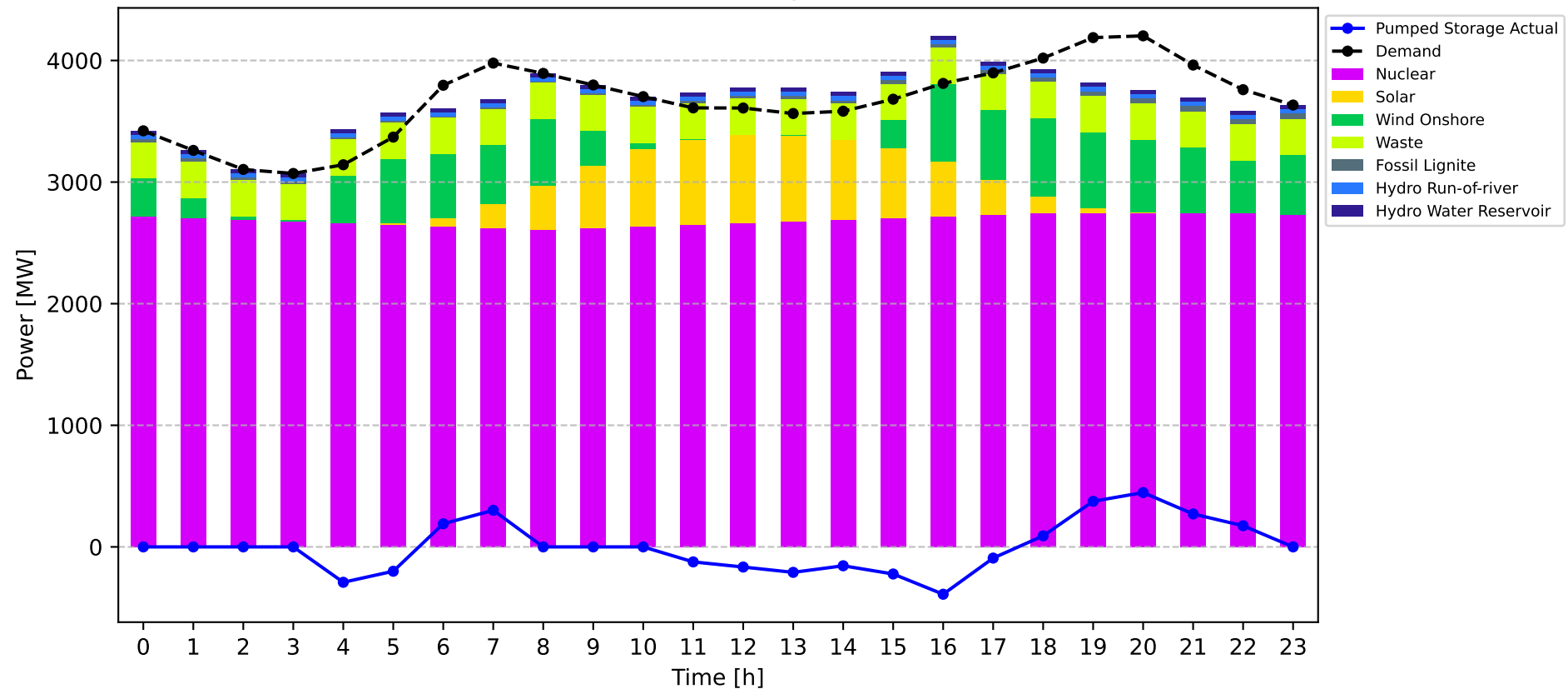
Optimal Energy Generation Dispatch Summer -- Day 4
