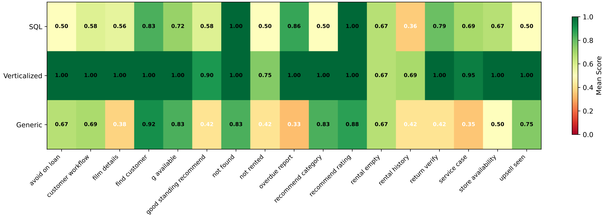
Per-Task Accuracy Heatmap
