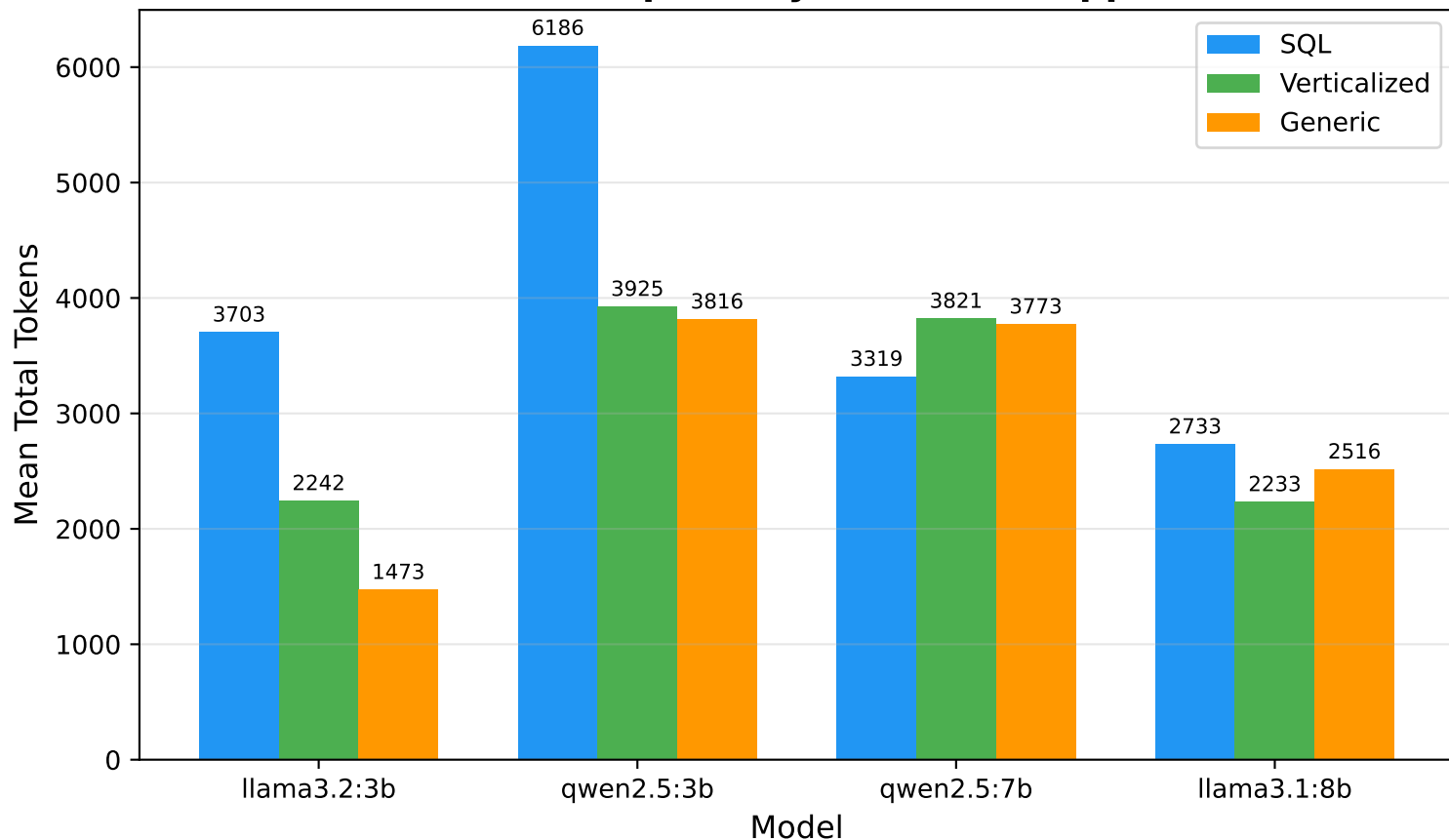
Token Consumption by Model and Approach
