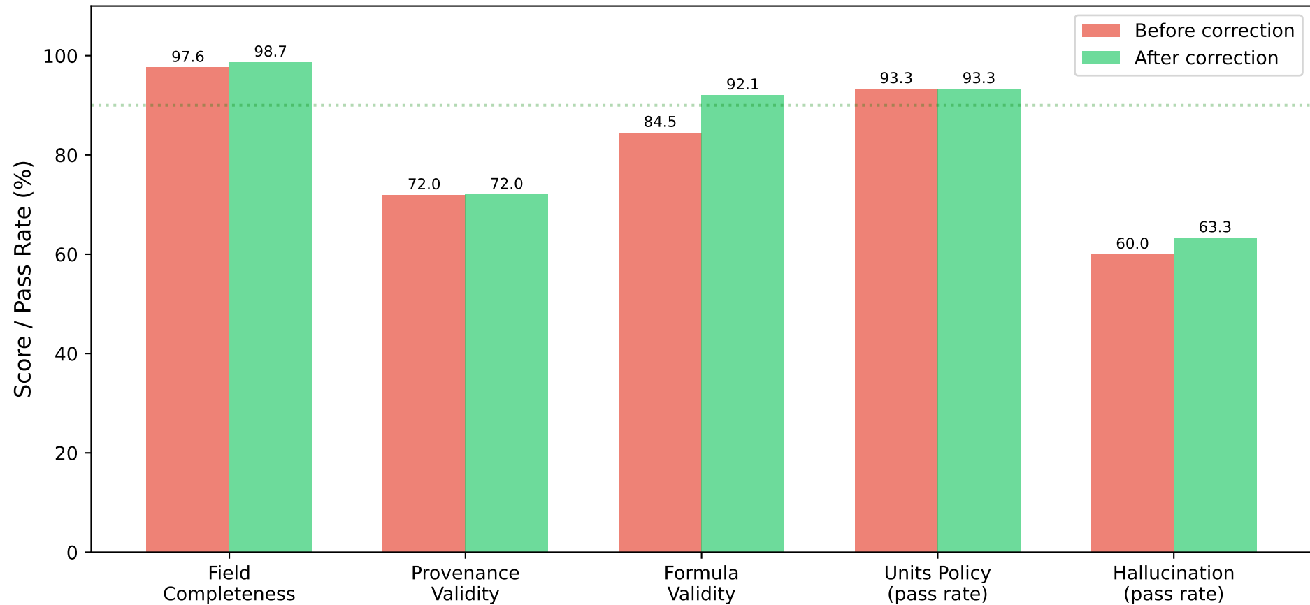
Evaluation Metric Breakdown: Before vs. After Correction
