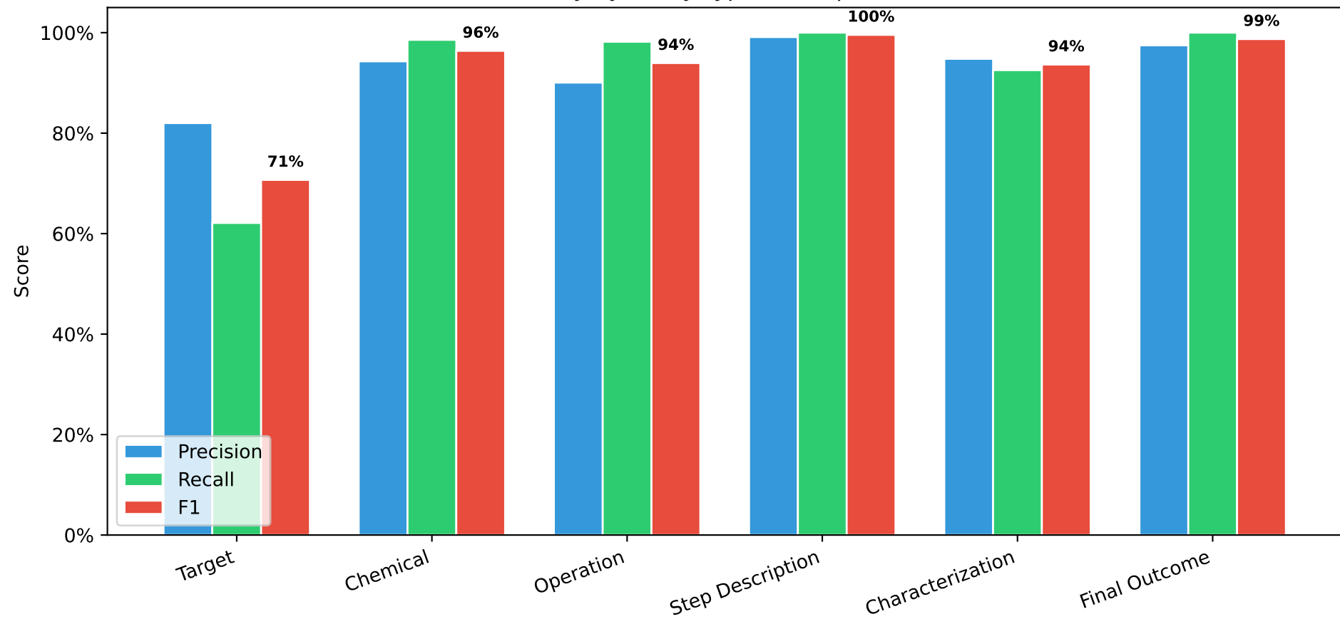
Extraction Quality by Entity Type (30-Paper Golden Dataset)
