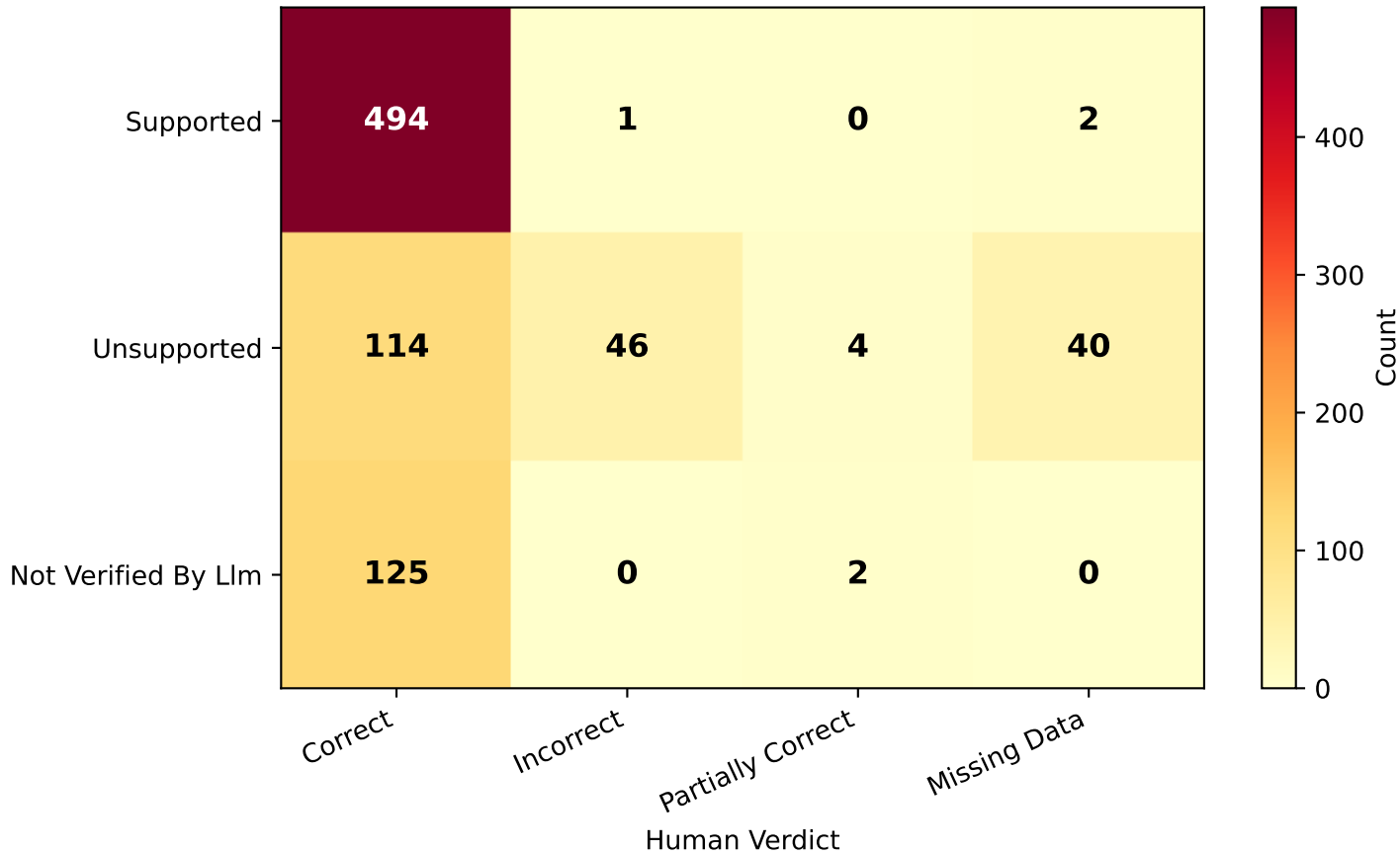
LLM Verifier vs. Human Expert: Confusion Matrix
