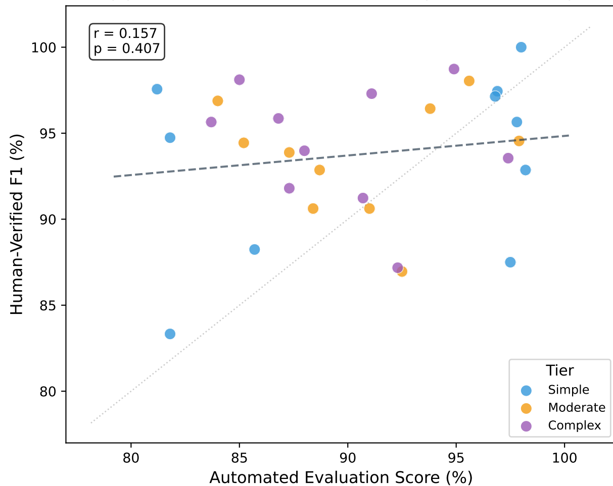
(a) Automated Score vs. Human F1 (After Correction)
