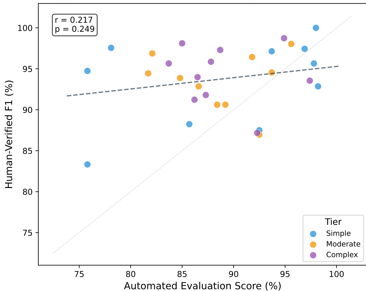
(b) Automated Score vs. Human F1 (Before Correction)
